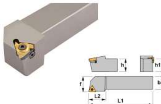
STXNR2525M16
