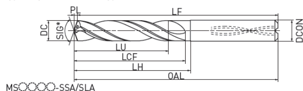
Type 1 Cylindrical shank type
